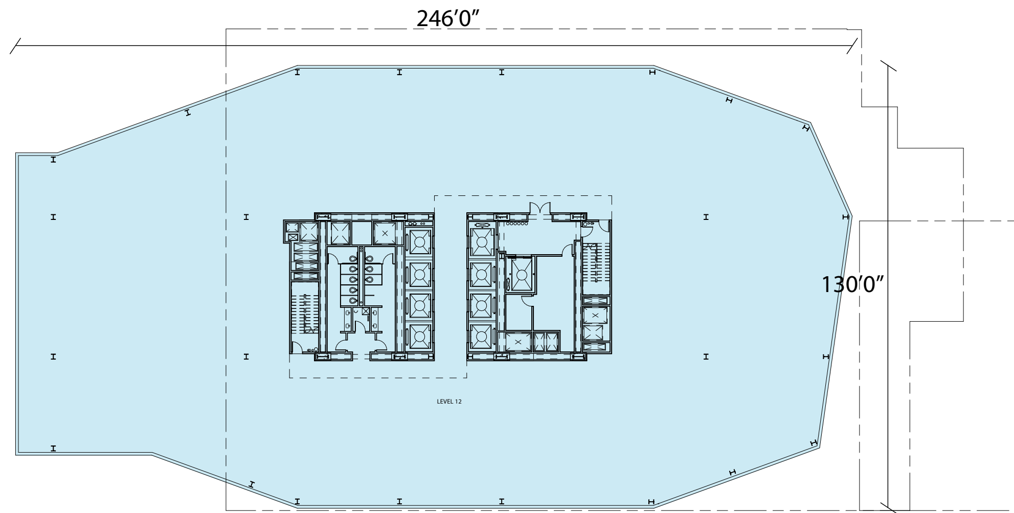
Level 12 - 27K GFA Office
