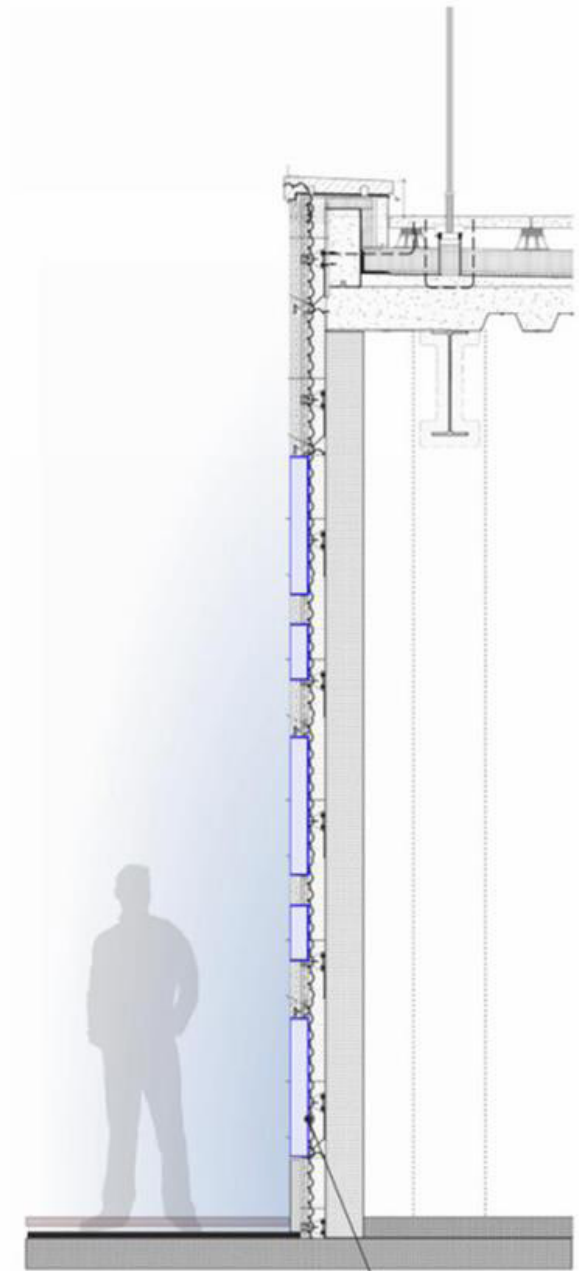
INTERSPERSED EXTERIOR GRADE SCREENS, INTEGRATED FLUSH WITH TERRA COTTA TILES (5000+ NIT, 192mm x 192mm LED MODULES)
