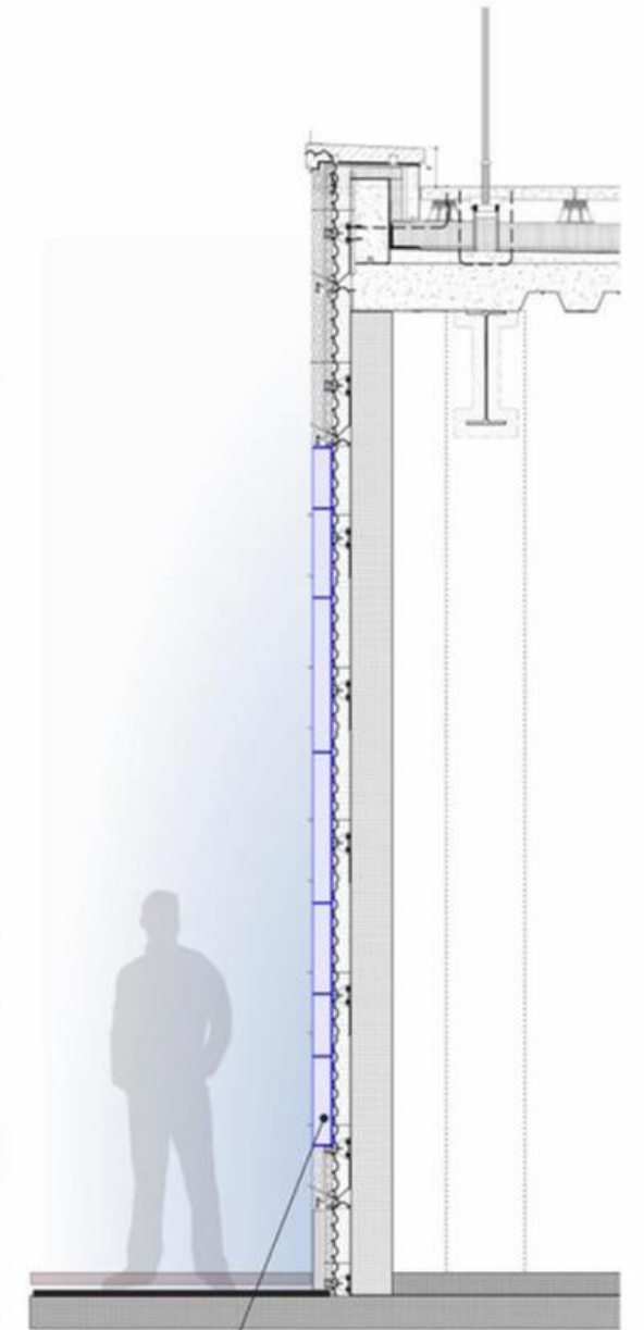
COMBINED EXTERIOR GRADE SCREENS, INTEGRATED FLUSH WITH TERRA COTTA T (28" x 15" LED SCREENS)
