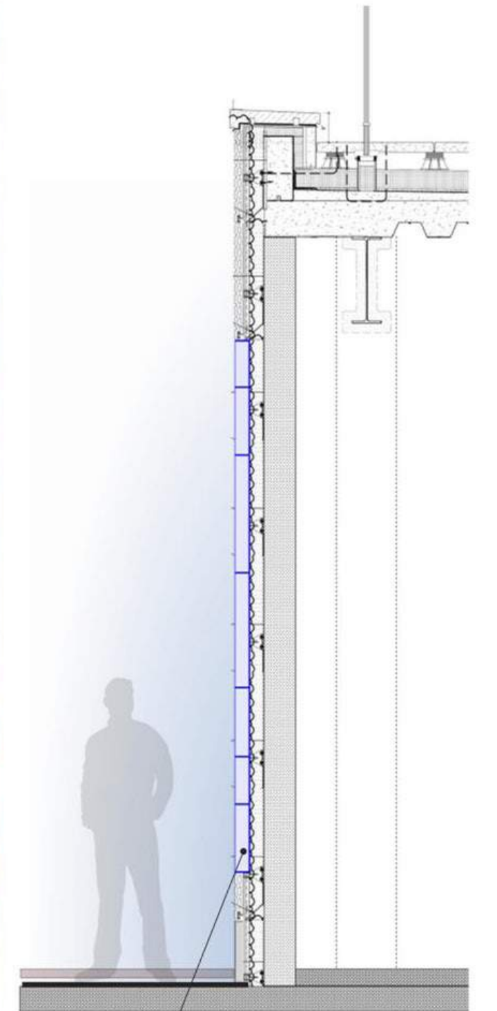
COMBINED EXTERIOR GRADE SCREENS, INTEGRATED FLUSH WITH TERRA COTTA T (28" x 15" LED SCREENS)
