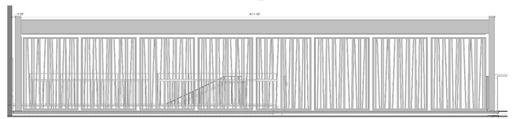
5 PANEL DETAIL ELEVATION BI-FOLD OPTION 2 PR7.02 1 1/2\"/>
