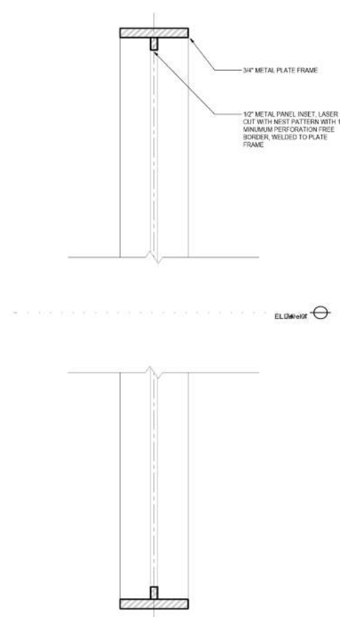
6 GATE PANEL SECTION - BI-FOLD OPTION 2 PR7.02 3\"/>
