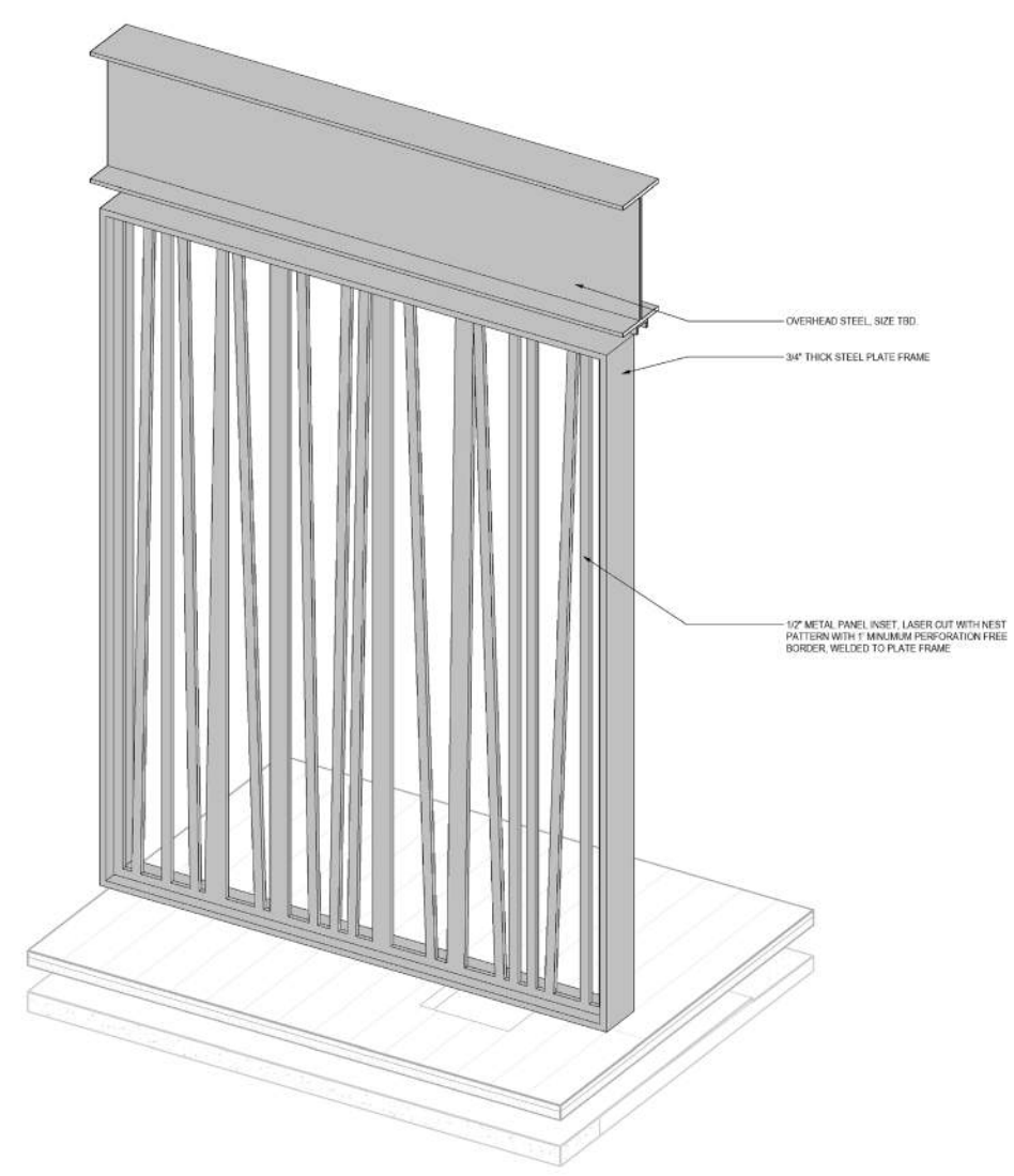
1 GREEN GARAGE GATE PANEL STUDY BI-FOLD OPTION 2 3D PR7.02
