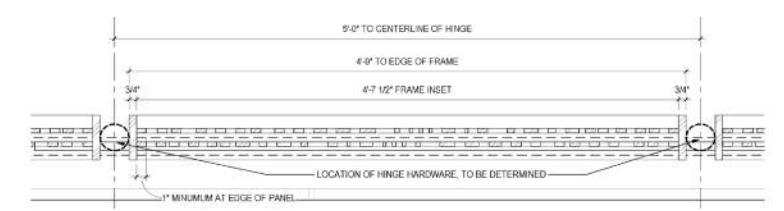
4 DETAIL PLAN - BI-FOLD OPTION 2 PR7.02 1 1/2\"/>
