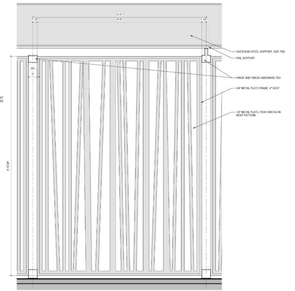
5 PANEL DETAIL ELEVATION BI-FOLD OPTION 2 PR7.02 1 1/2\"/>
