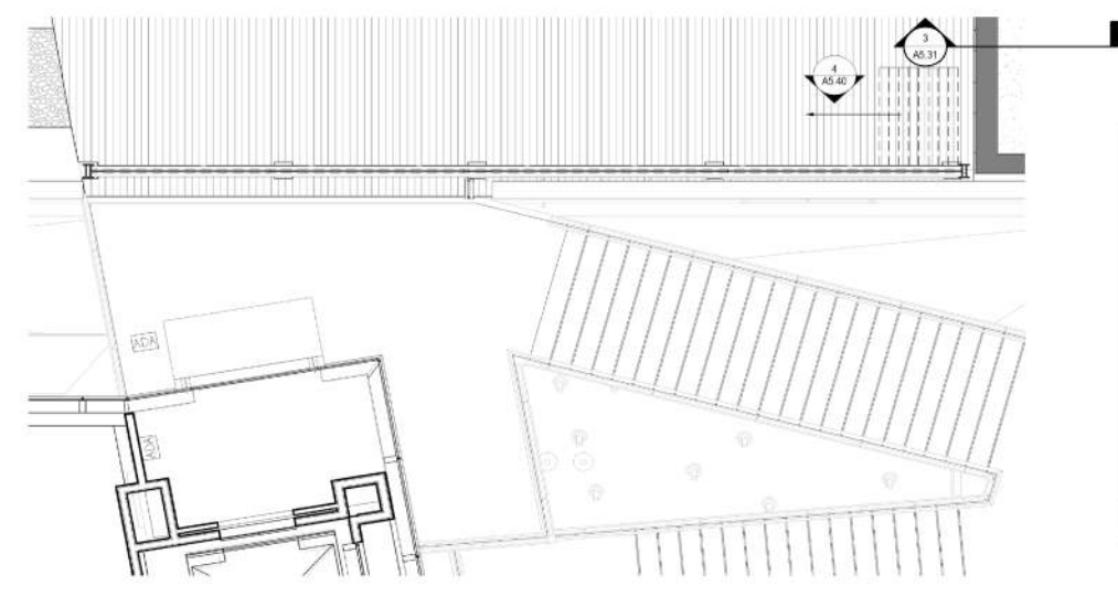
2 OVERALL PLAN - BI-FOLD OPTION 2 PR7.02 1/4\"/>
